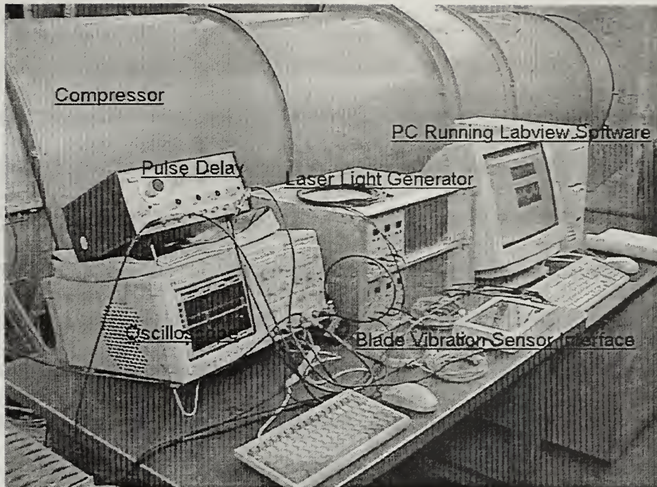
Figure 2.5 Test apparatus showing data acquisition equipment.
